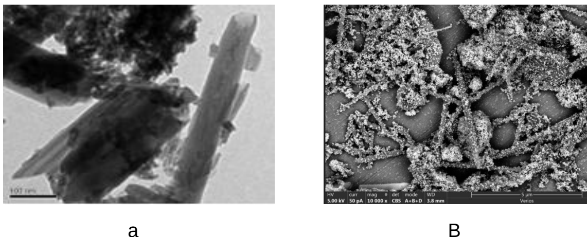
Fig. SEM images of HNTs (Sigma Aldrich)with incorporated into lumens MnOOH (a), HNTs (UltraPure) (b) decorated by NPs of Mn_3O_4 in phase contrast mode with magnification \times 10\,000 .
